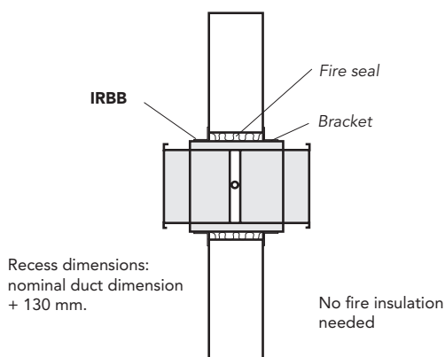
Installation in structural element
