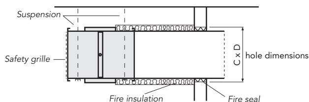
Installation away from structural element
